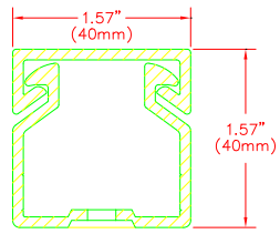
FRONT SECTION
